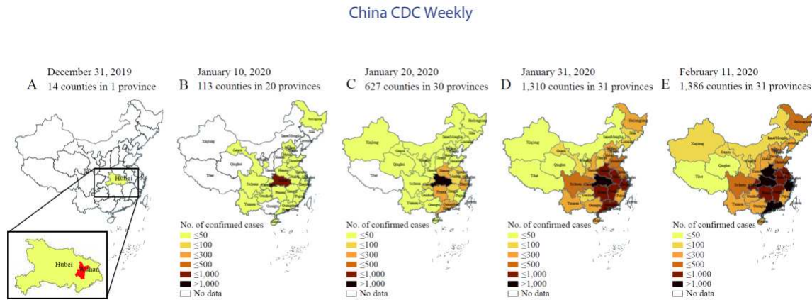
Figure 22. Geo-temporal spread of COVID-19 in China through February 11, 2020. (A) a total of 14 county-level administrative areas (hereafter counties) in Hubei Province only (inset) had reported cases as of December 31, 2019; (B) by January 10, 2020, 113 counties in 20 provincial level administrative divisions (PLADs) had reported cases with the highest prevalence still in Hubei Province; (C) nine days later, on January 20, 627 counties in 30 PLADs had reported cases and PLADs neighboring Hubei Province observed increasing prevalence; (D) by the end of January 31, 1,310 counties across all 31 PLADs were affected and prevalence in the central, south, and south-central regions had risen dramatically; (E) by the end of February 11, 2020 1,386 counties nationwide were affected and prevalence in the south-central PLADs had risen to the level of Hubei. Source: The Epidemiological Characteristics of an Outbreak of 2019 Novel Coronavirus Diseases (COVID-19) — China, 2020. China CDC Weekly . 2020;2(8):113-122. https://doi.org/10.46234/ccdcw2020.032
